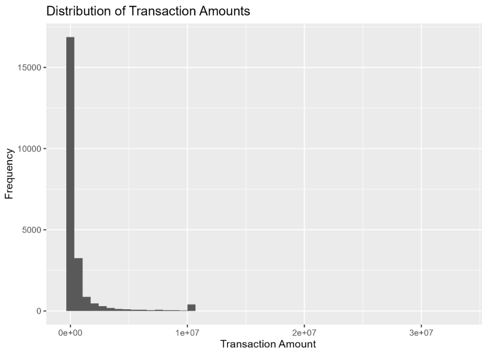
Figure 2.4: Distribution of transaction amounts.
